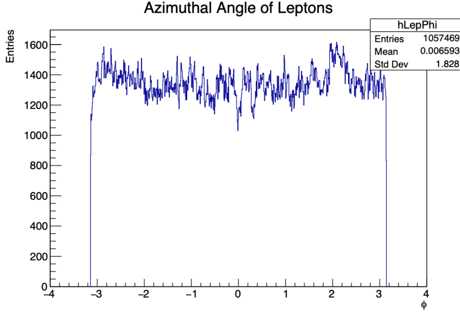
Figure 5: lep_phi graph
