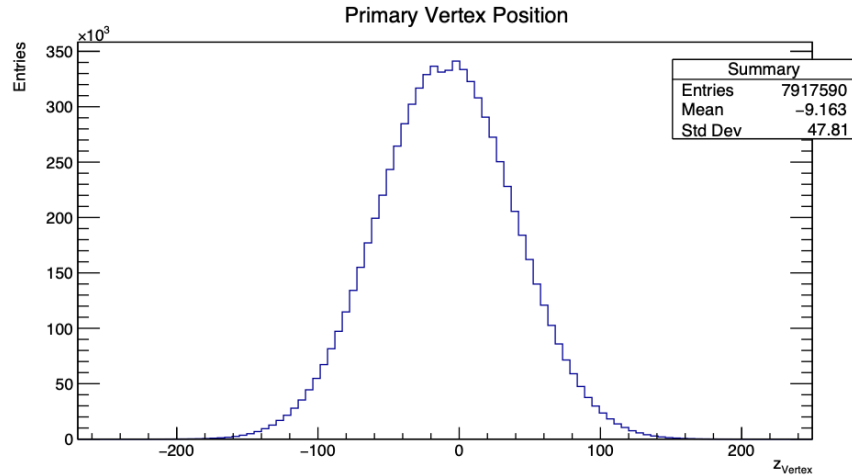
Figure 1: vxp_z graph
